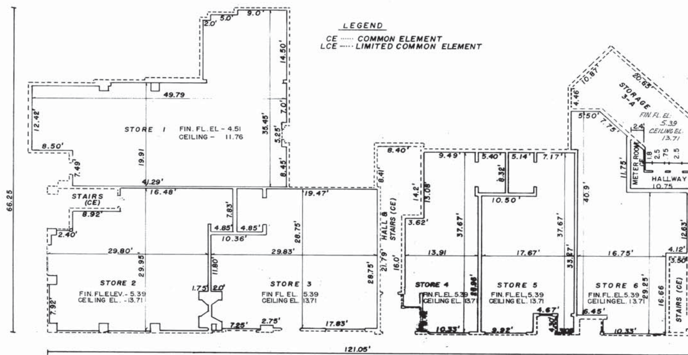
FIRST STORY FLOOR PLAN
