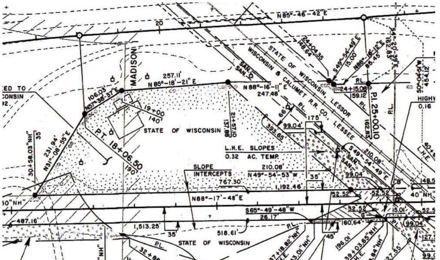
Part of Wisconsin D.O.T. survey of roads from 1985, including 30 Nob Hill Road site
