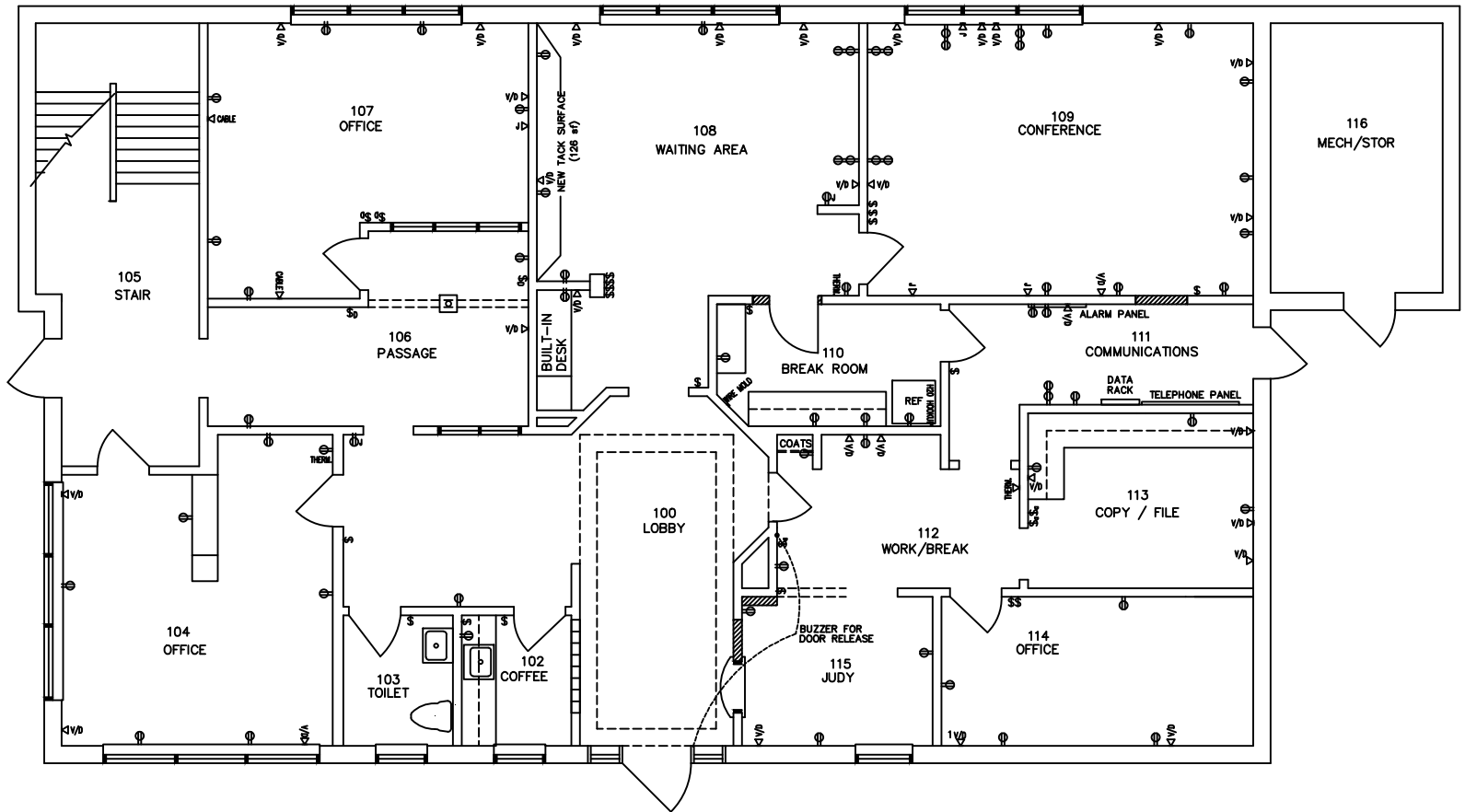
LEVEL 1 PLAN - 119 East 8th Street
