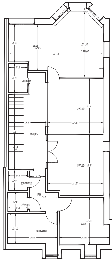
4TH FLOOR
