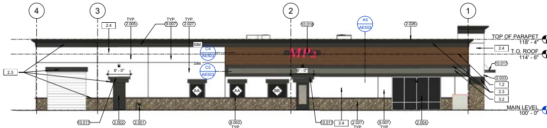
A1 NORTH BUILDING ELEVATION 1/8" = 1'-0"
