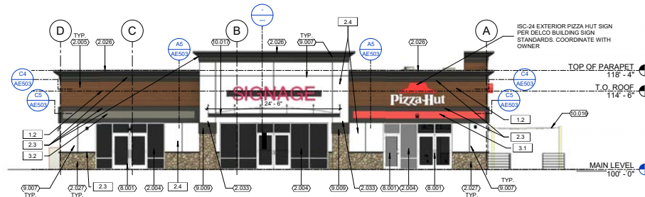
B1 WEST BUILDING ELEVATION 1/8" = 1'-0"
