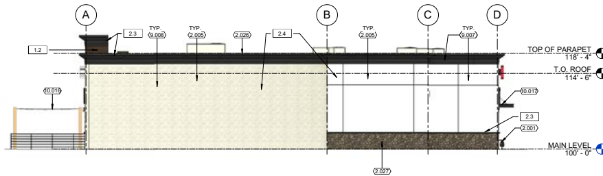
C1 EAST BUILDING ELEVATION 1/8" = 1'-0"
