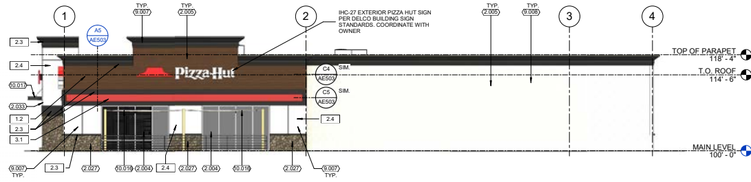
D1 SOUTH BUILDING ELEVATION 1/8" = 1'-0"
