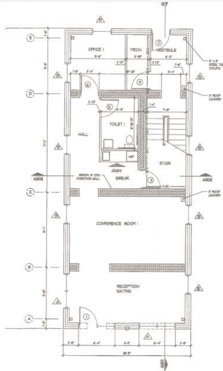
A101 NEW FIRST FLOOR PLAN Scale: 1/4" = 1'-0"
