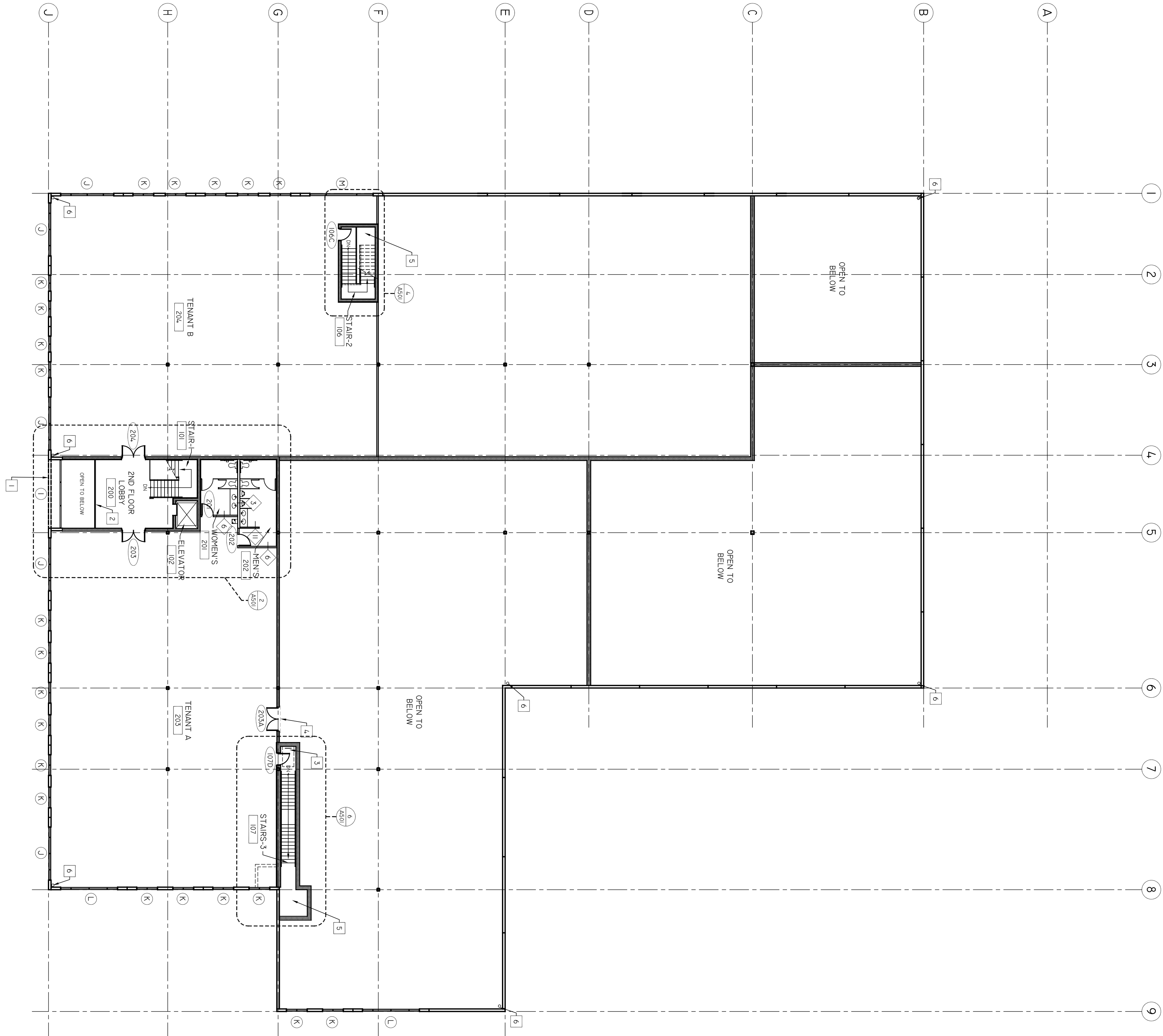
1 2ND FLOOR PLAN A102 1/16" = 1'-0"
