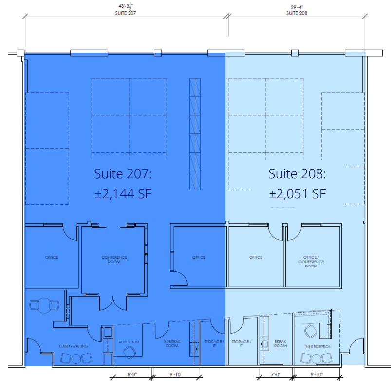
Conceptual demising and modification plan
