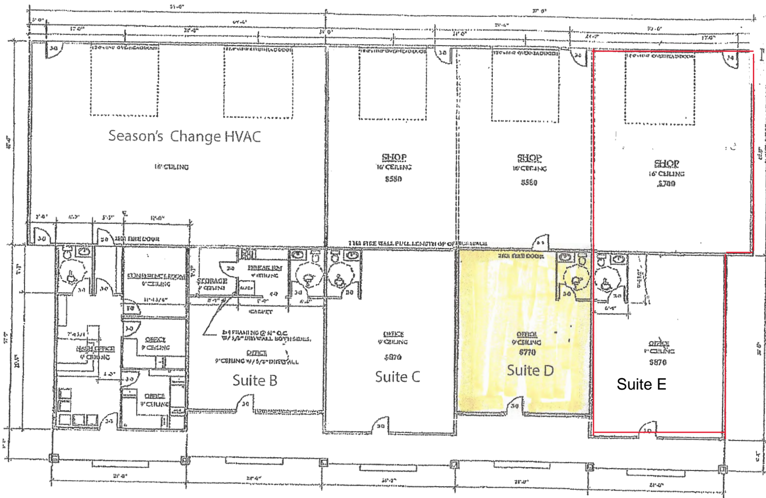
Floor Plan Beacon Hill Land Flex Building 2815 Laverne
