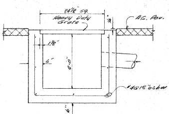
TYP. CATCH BASIN
