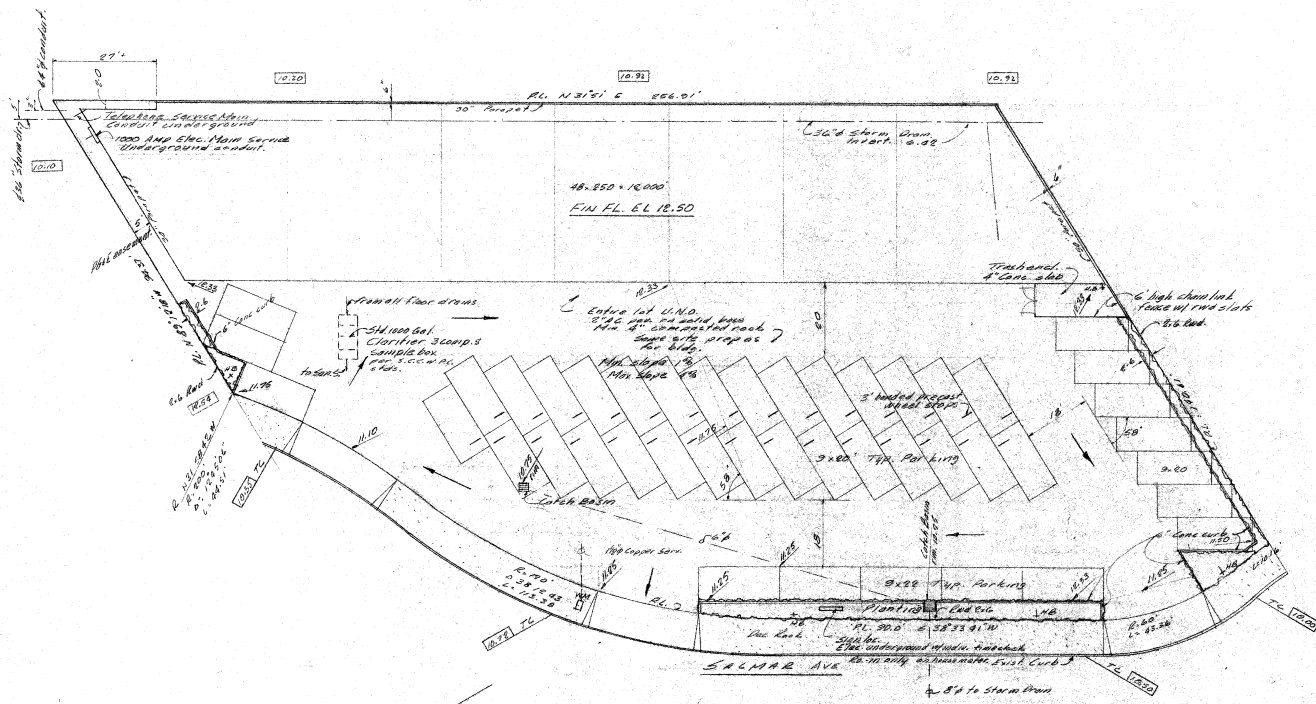
SITE PLAN Scale 1/4" = 1'-0"
