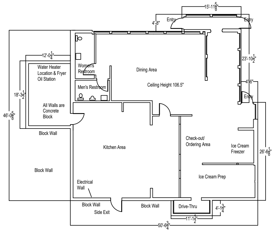
DAIRY QUEEN 5608 Outer Loop, Louisville KY 40219 EXISTING FLOORPLAN WITH OUTSIDE DIMENSIONS
