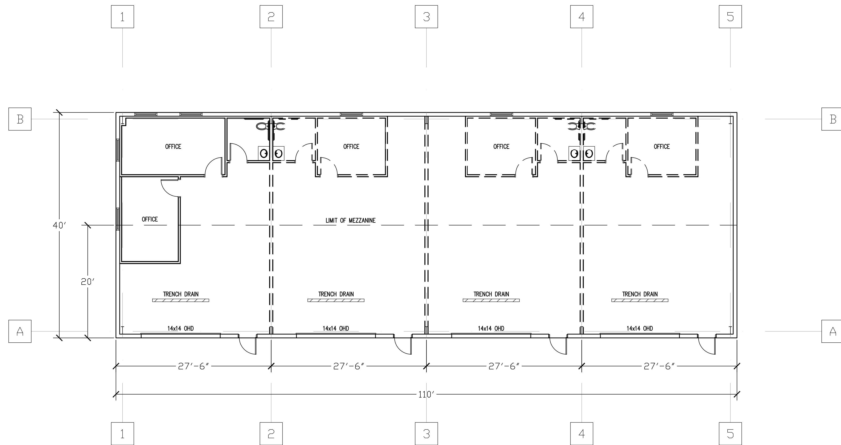
FLOOR PLAN
