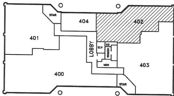
KEY PLAN-BUILDING 1506 FOURTH FLOOR PLAN
