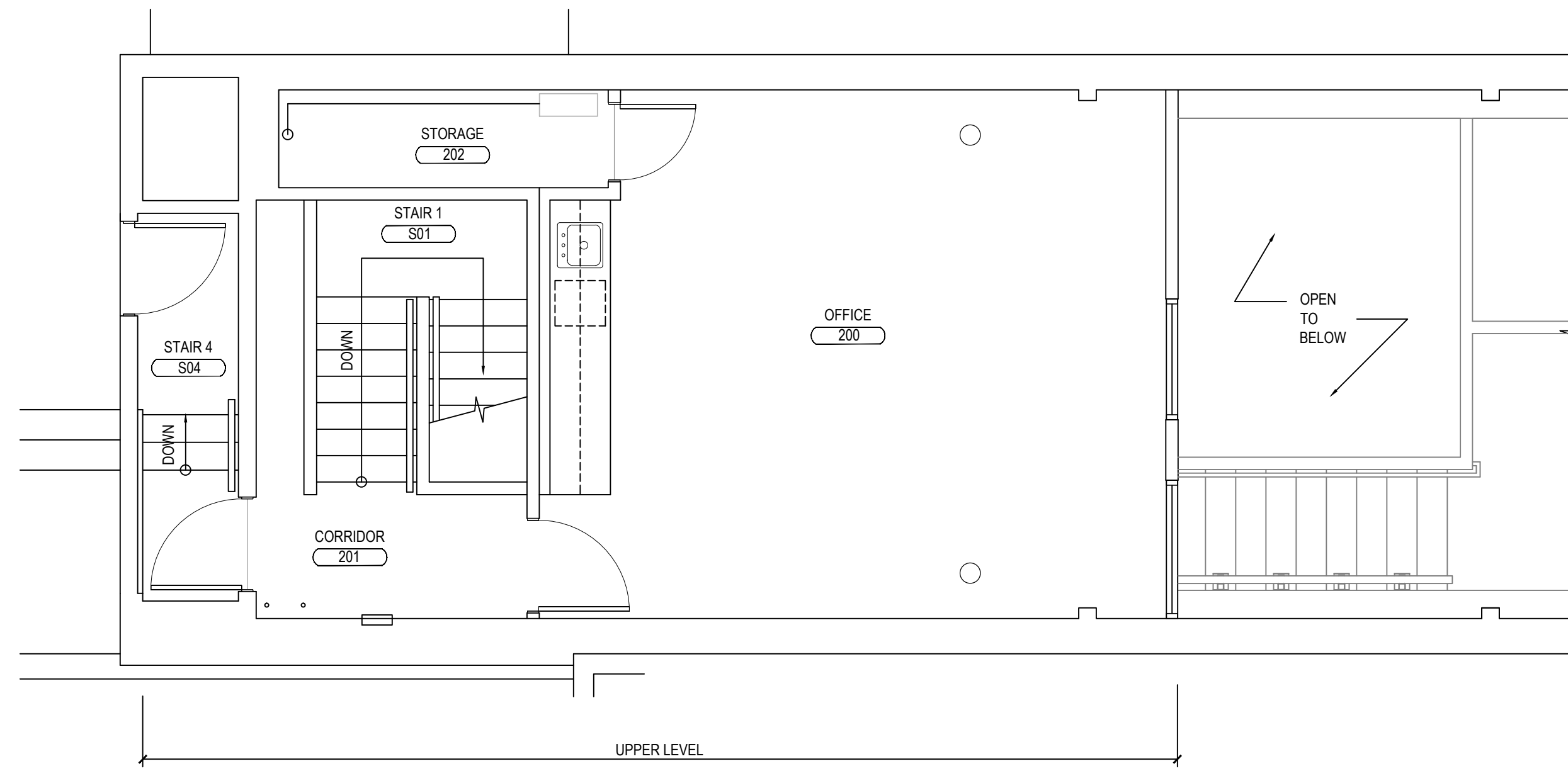
2 UPPER LEVEL FLOOR PLAN 1/4" = 1'-0"
