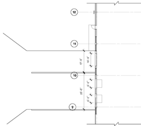
ENLARGED DOCK PLAN
