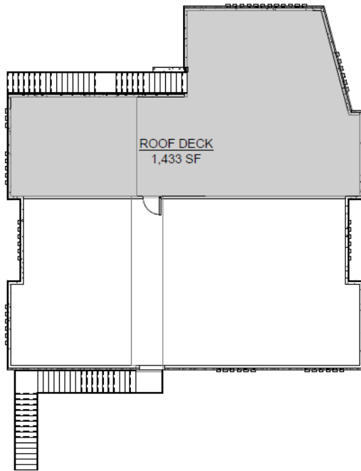
3 ROOF DECK A0.0 SCALE: 1/16" = 1'-0"
