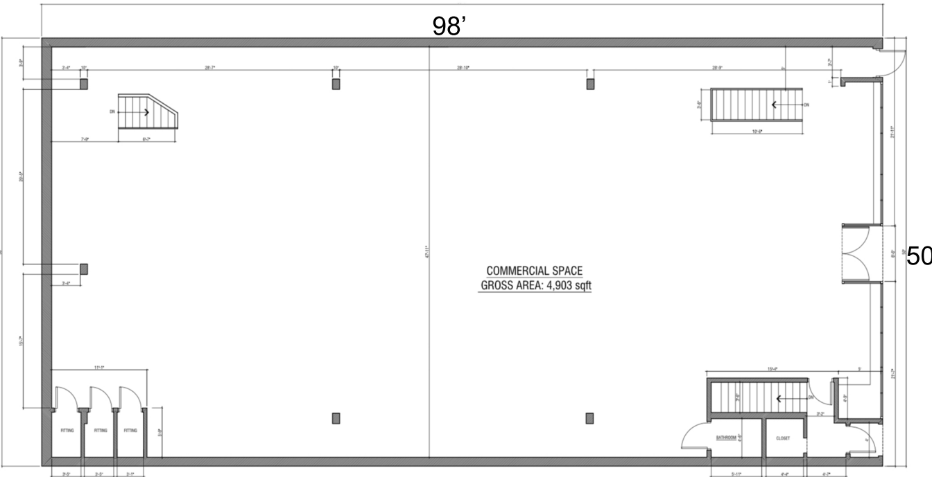
1 EXISTING 1ST FLOOR PLAN Scale: 1/8" = 1'-0"
