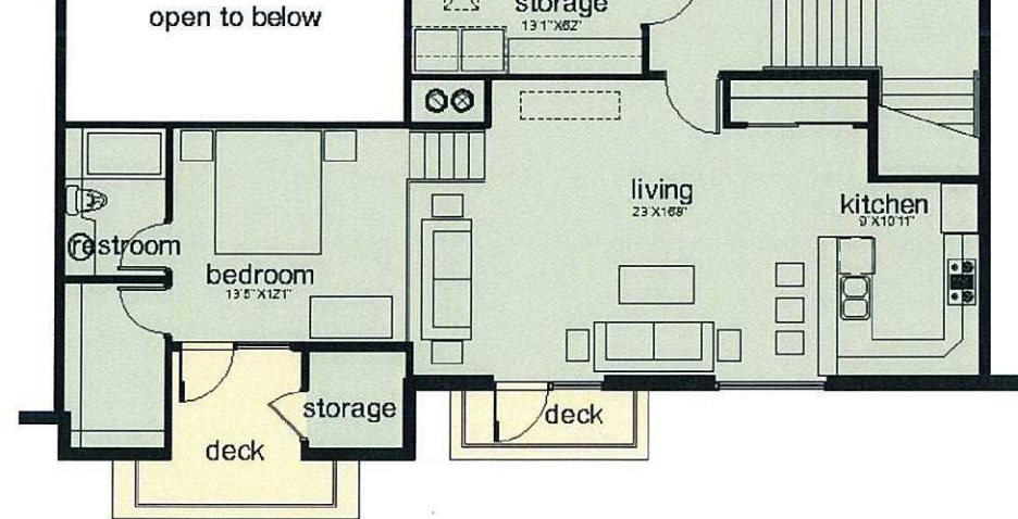
2nd Floor Plan - Building 'C1'
