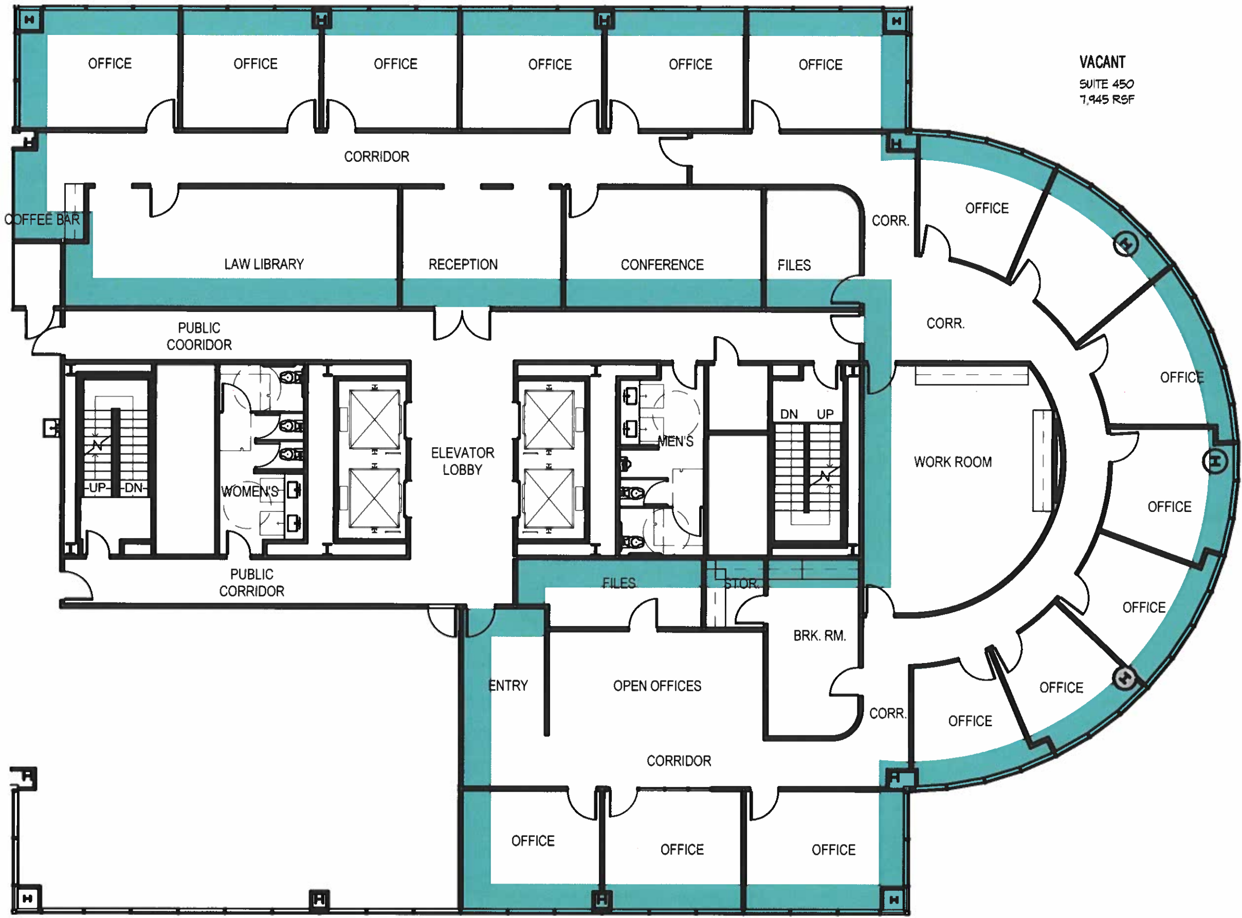
4th Floor Plan - Suite 450
