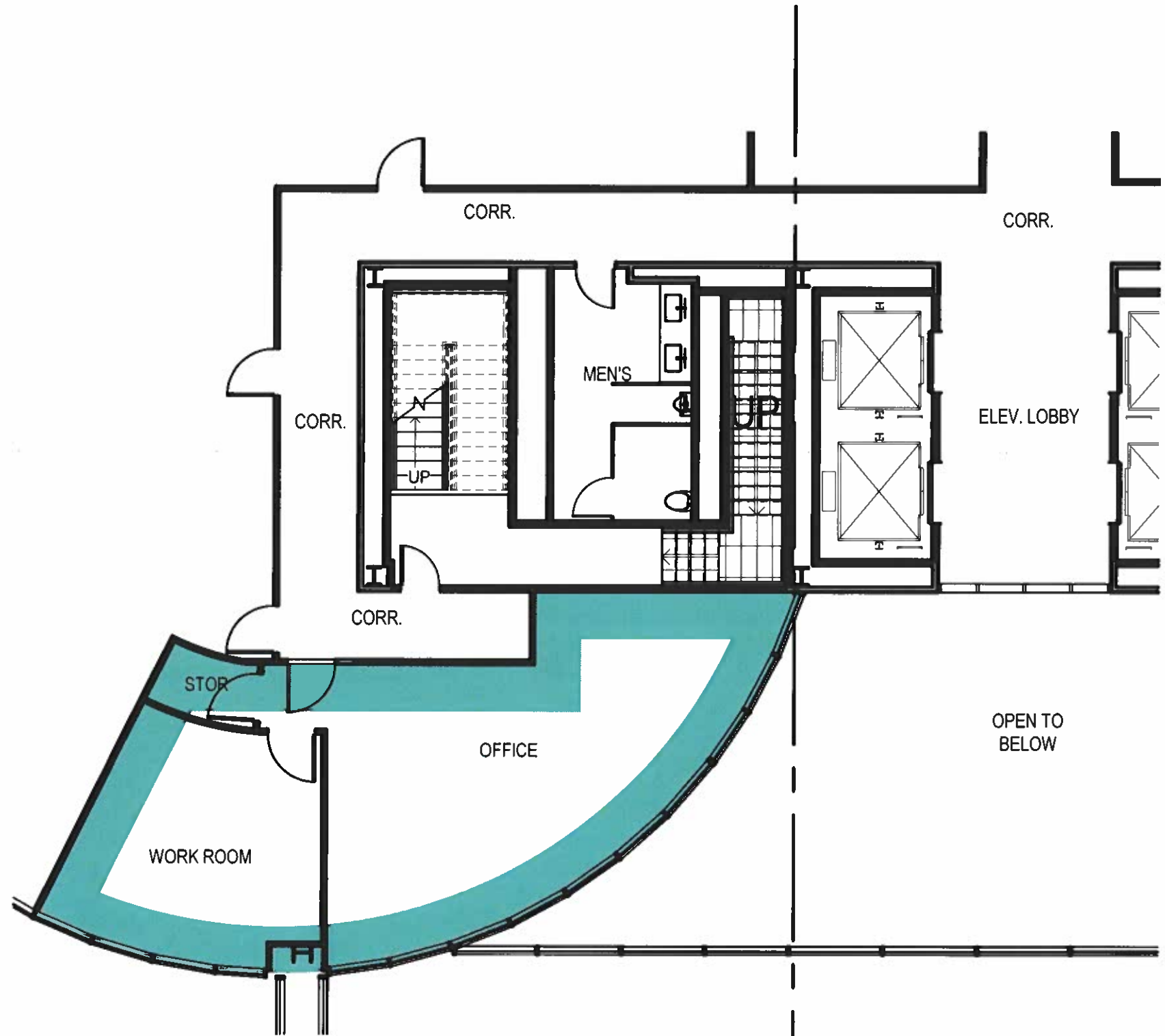
2nd Floor Plan - Suite 210
