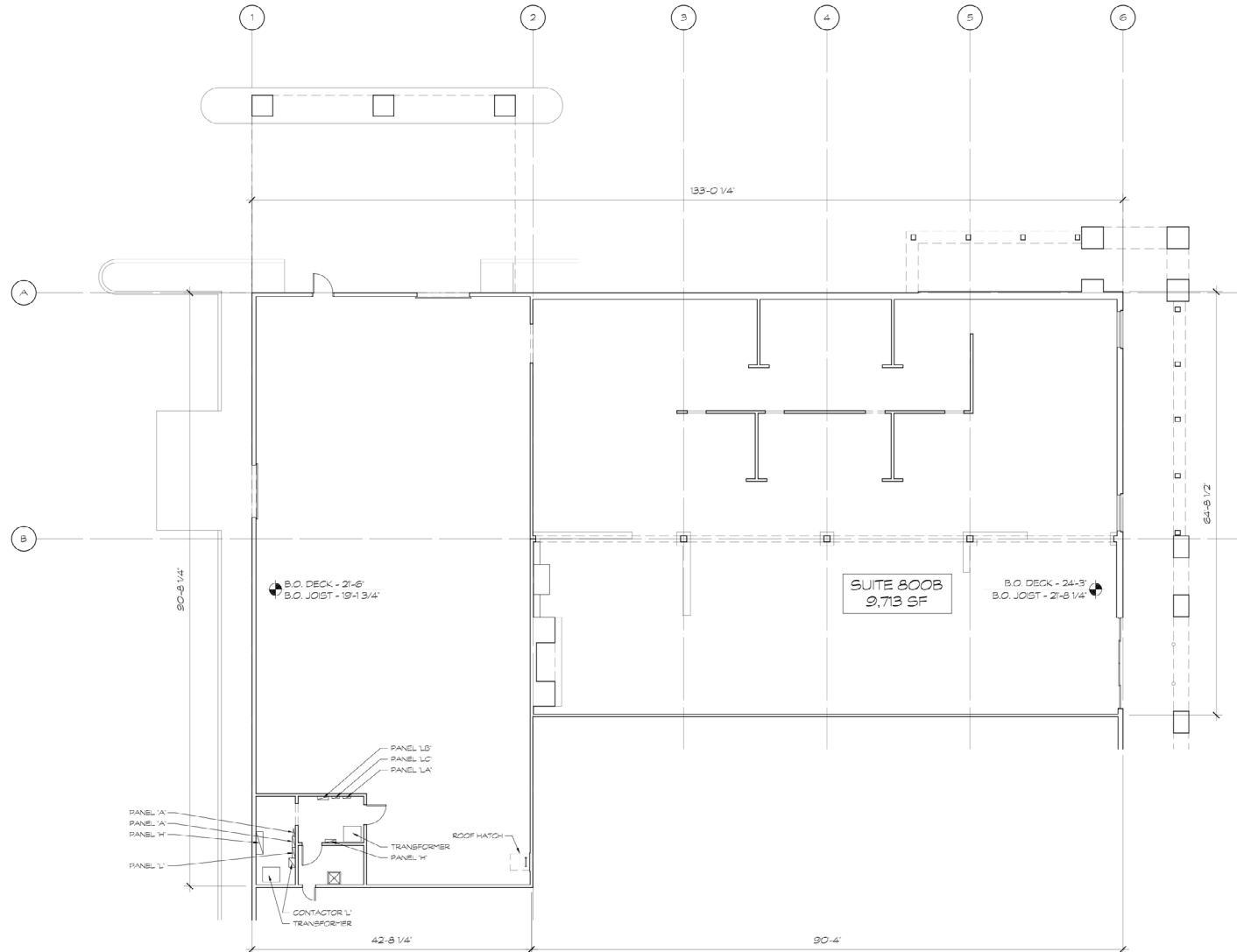
1 LEASING PLAN - SUITE 800B 3/32" = 1'-0" 388-06-01 Leasing Plan - Suite 800B 01-01
