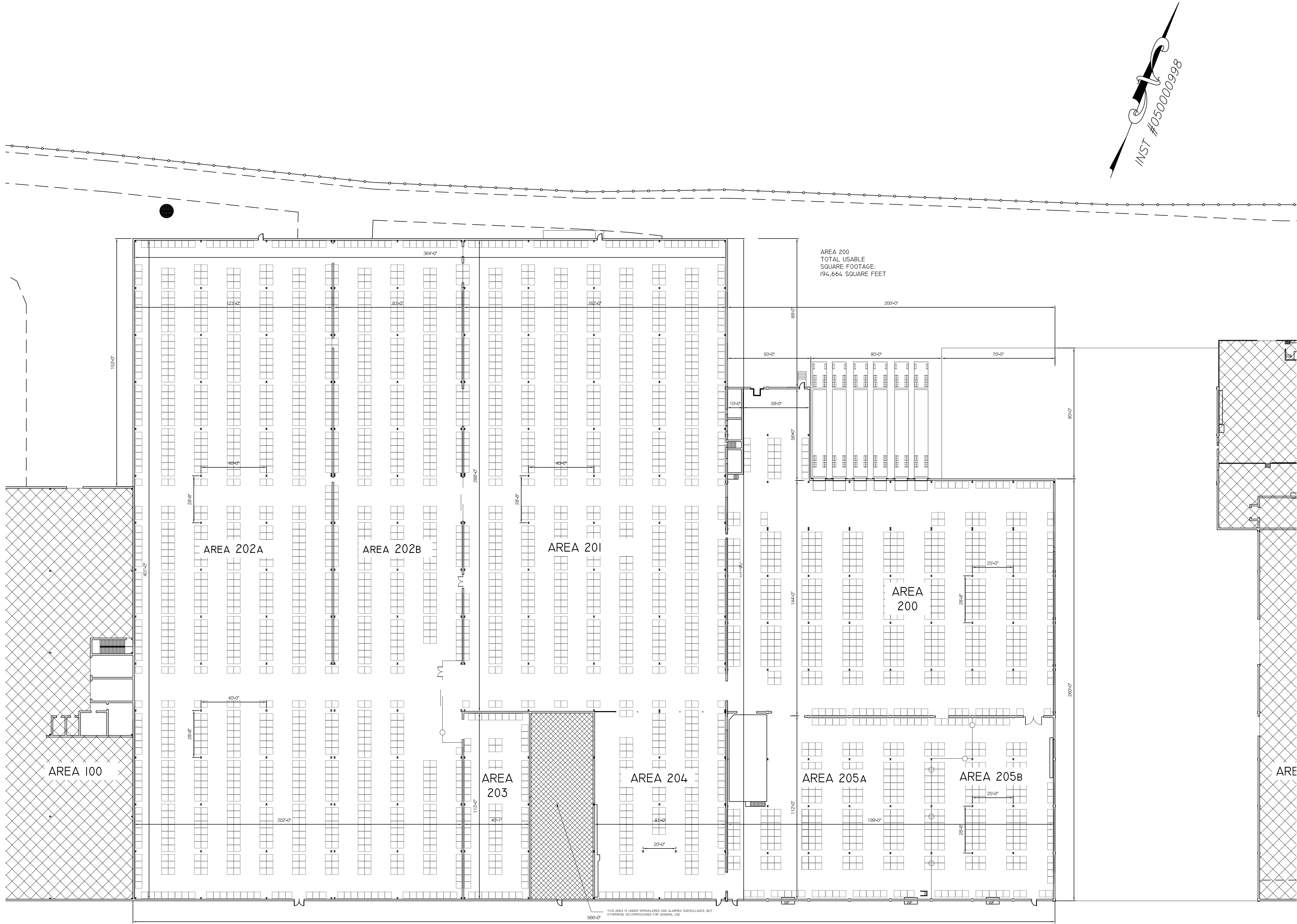
1 AREA 200 STORAGE AREA LIFE SAFETY DIAGRAM SCALE: 1/32" = 1'-0"
