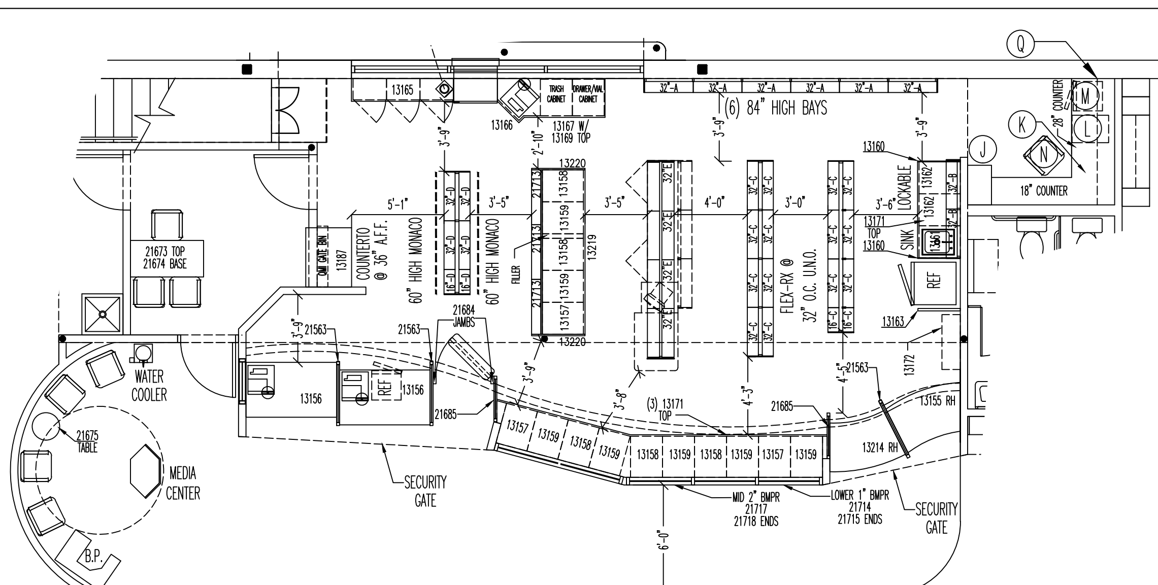
PHARMACY PLAN SCALE: 3/16" = 1'-0"
