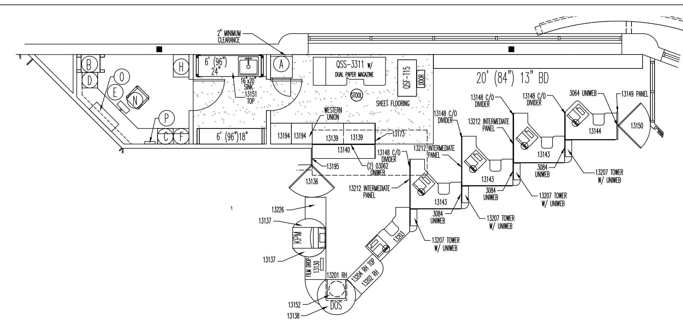
FRONT END PLAN SCALE: 3/16" = 1'-0"
