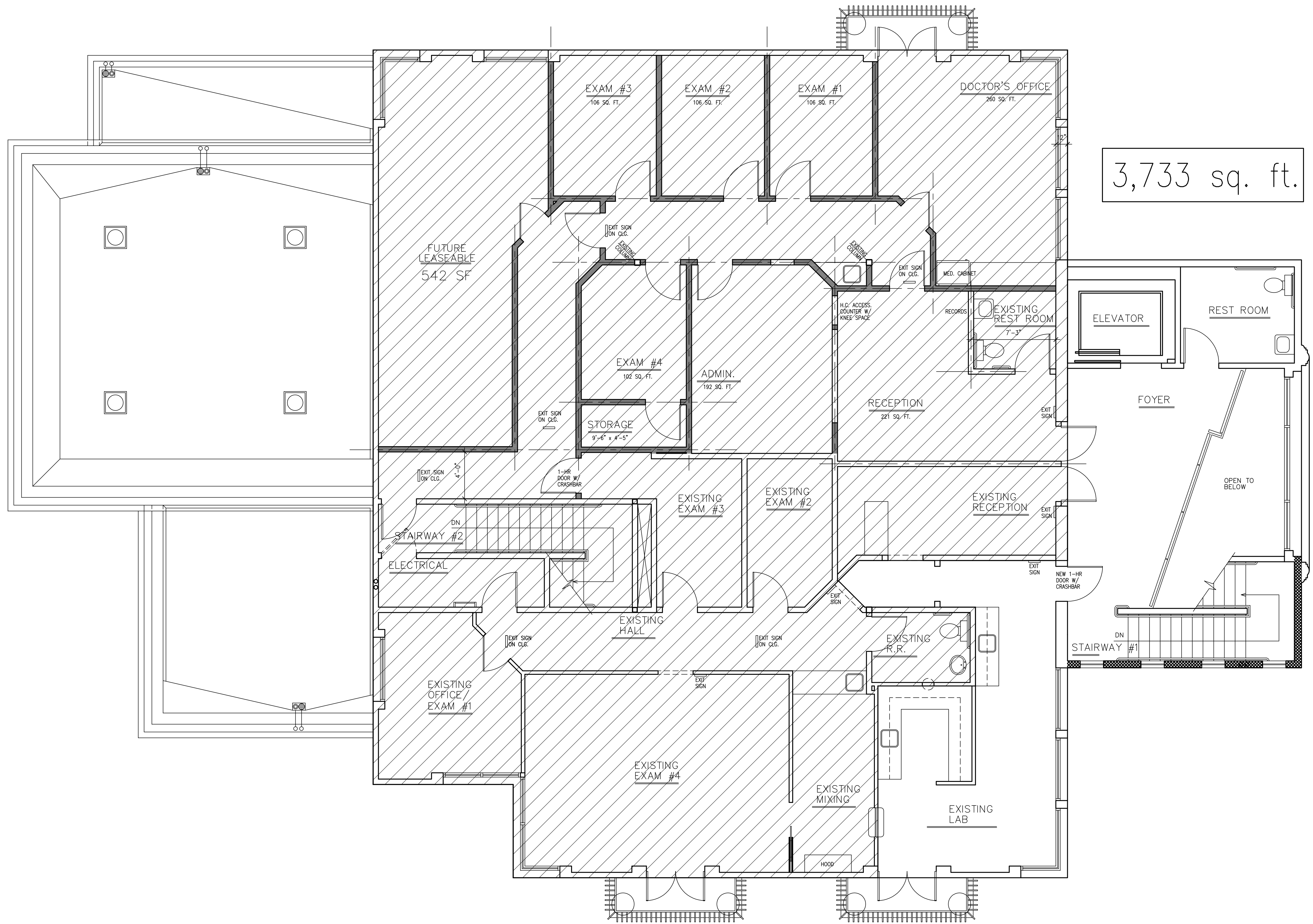
1 SECOND LEVEL FLOOR PLAN SCALE: 1/4"=1'-0"
