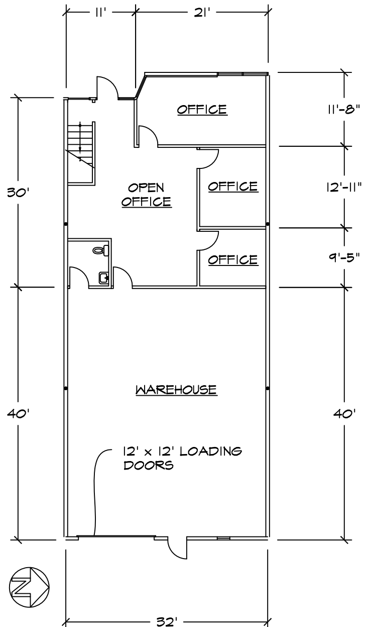
FIRST FLOOR
