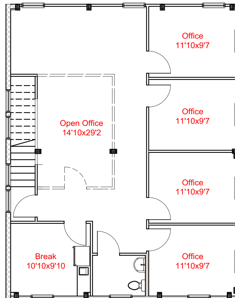
SECOND FLOOR PLAN 1,210 SQ. FT.
