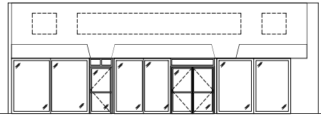
1. FRONT ELEVATION SCALE: 1/4" = 1'-0"
