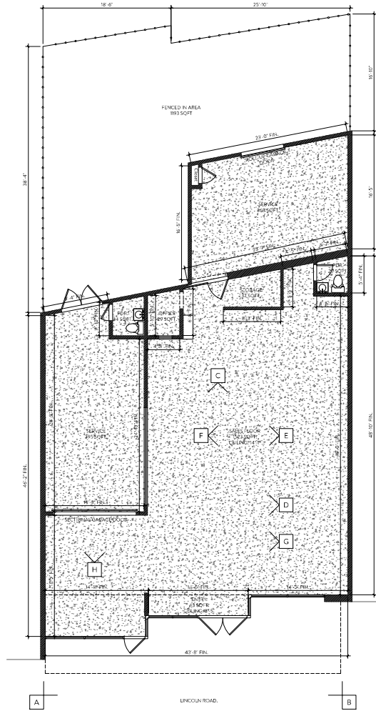
2. FLOOR PLAN SCALE: 1/4" = 1'-0"
