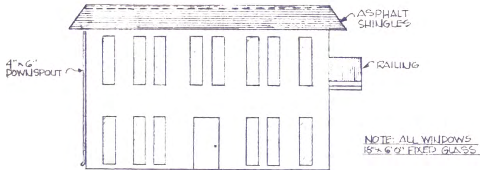
FRONT ELEVATION
