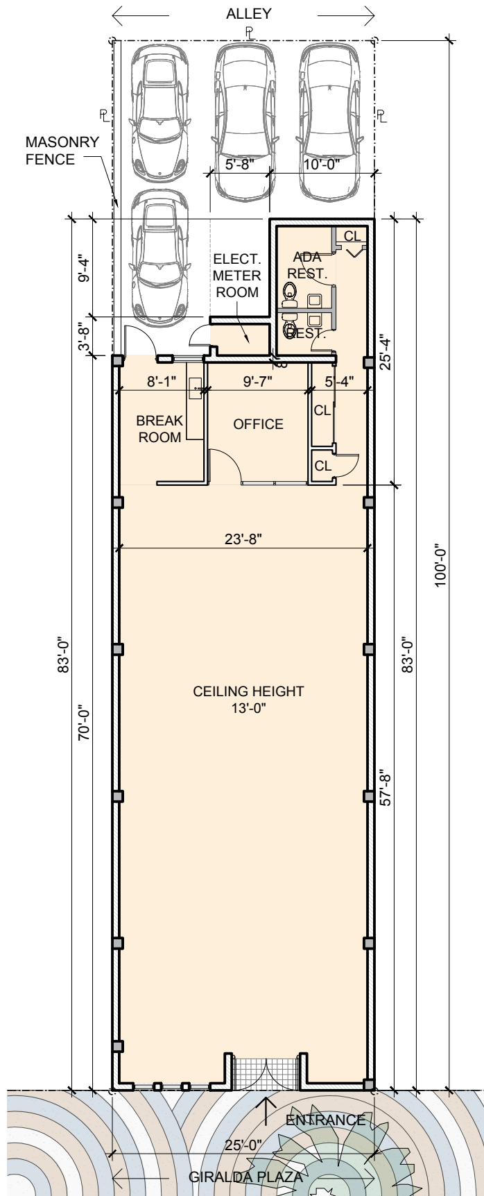
137 GIRALDA PLAZA FLOOR PLAN
