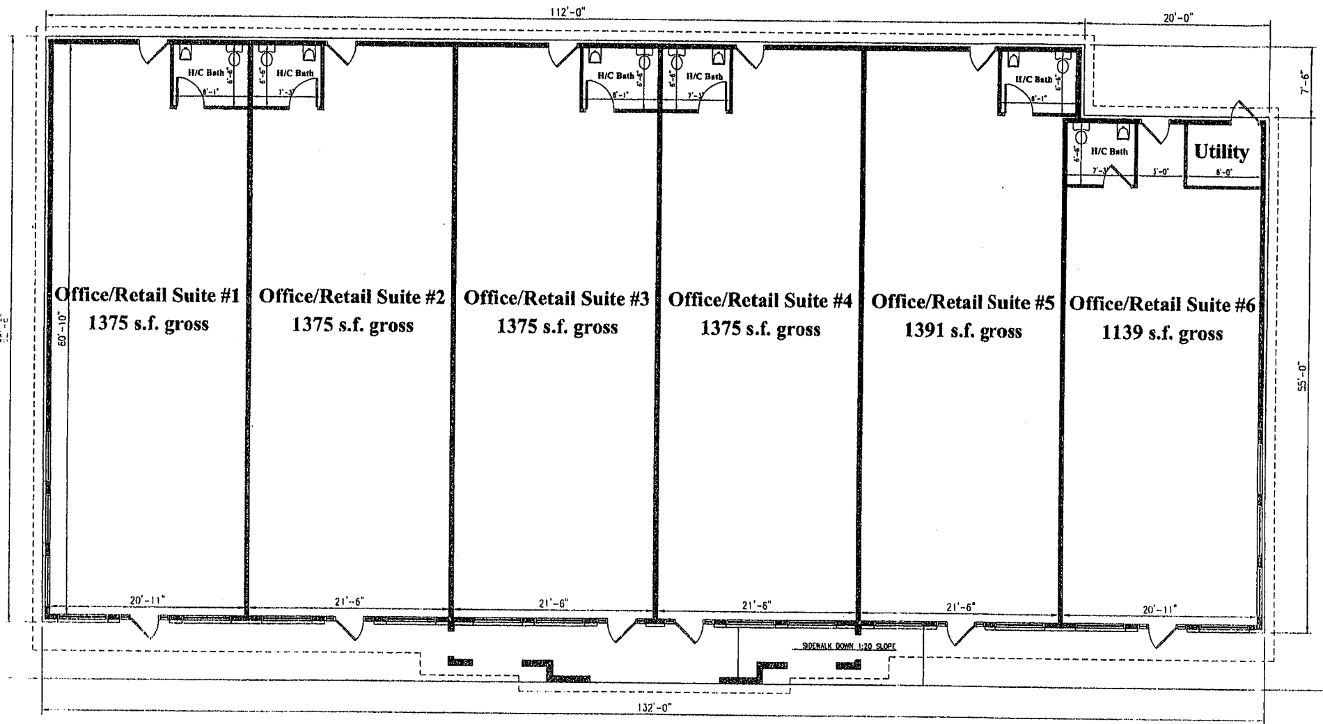
1 FIRST FLOOR PLAN A2 Scale: 3/16"=1'-0" 8100 S.F.
