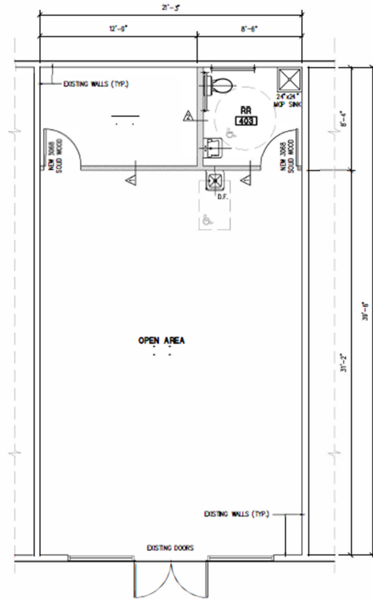
1 FLOOR PLAN SCALE: 1/4"=1'-0" NORTH
