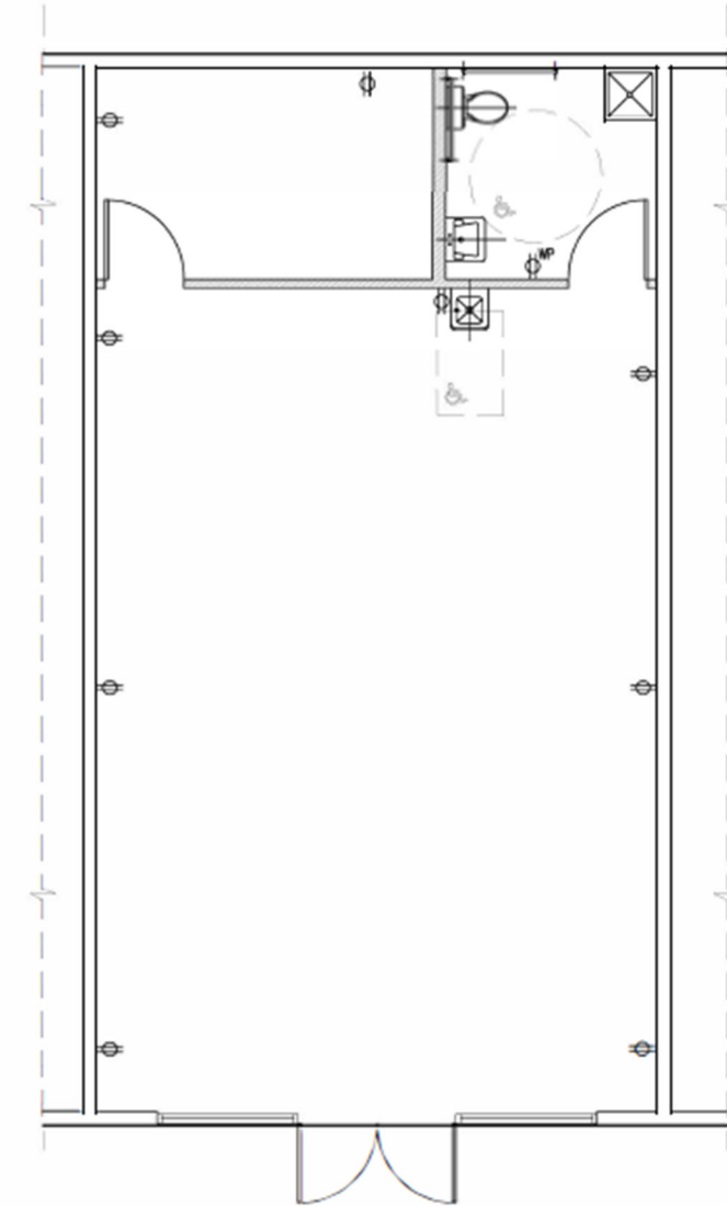
3 ELECTRICAL PLAN SCALE: 1/4"=1'-0" NORTH
