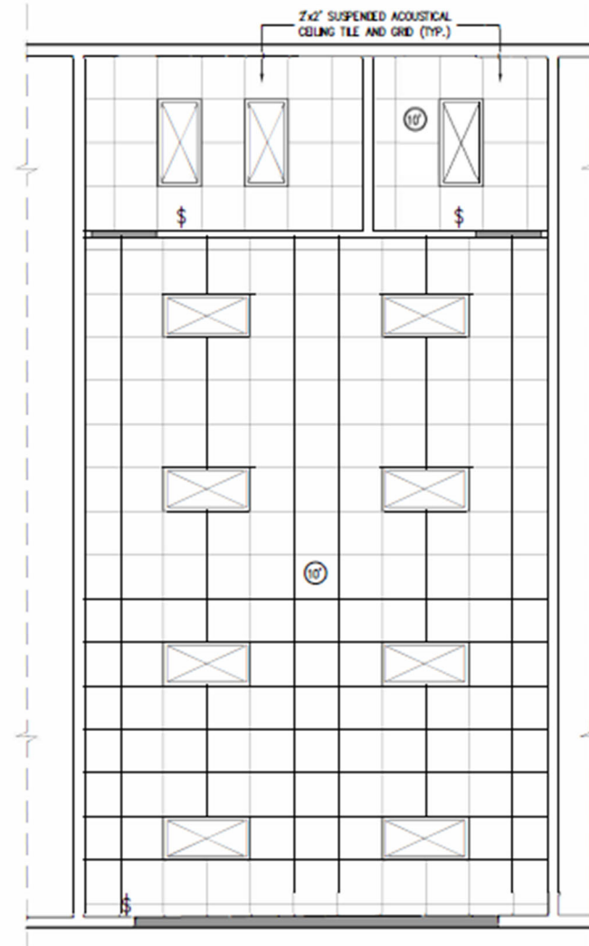
2 REFLECTED CEILING PLAN SCALE: 1/4"=1'-0" NORTH
