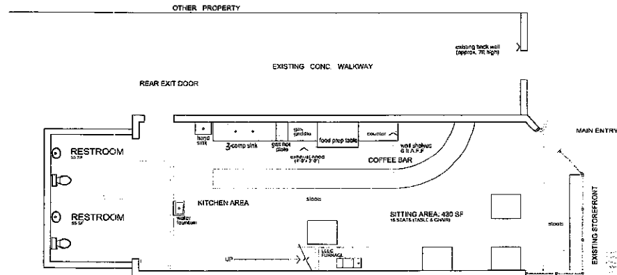
EXISTING FIRST FLOOR PLAN SCALE: 1/4"=1'-0"
