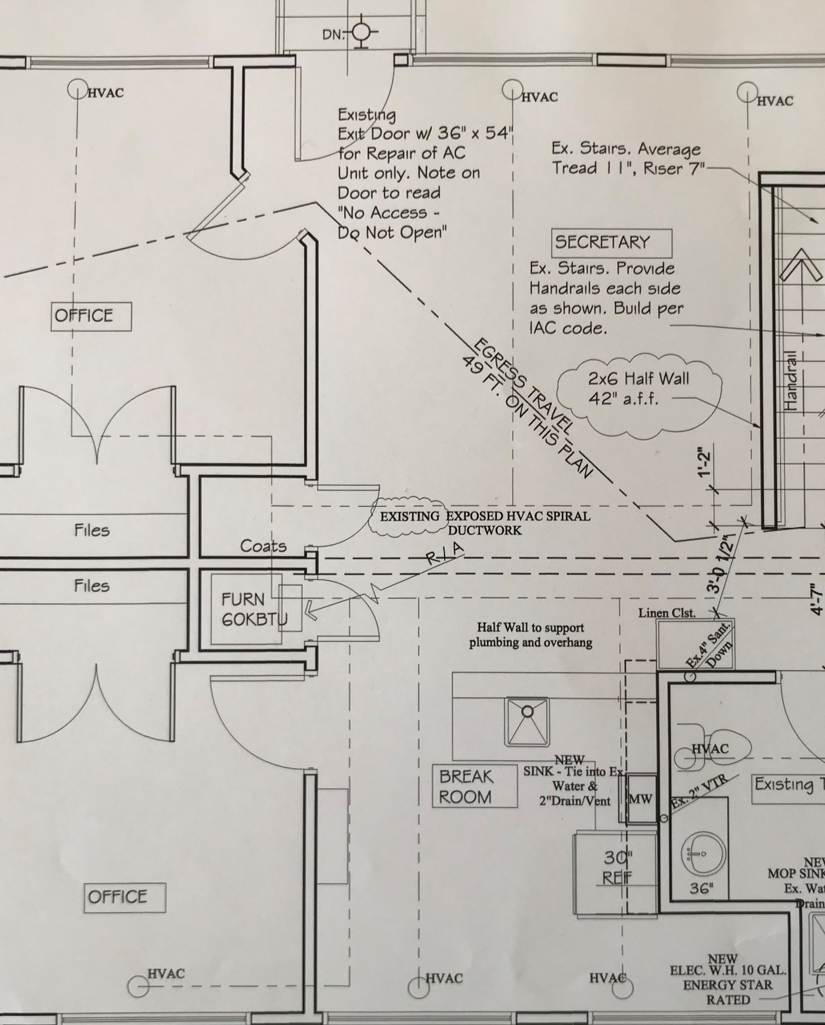
PER LEVEL FLOOR PLAN
