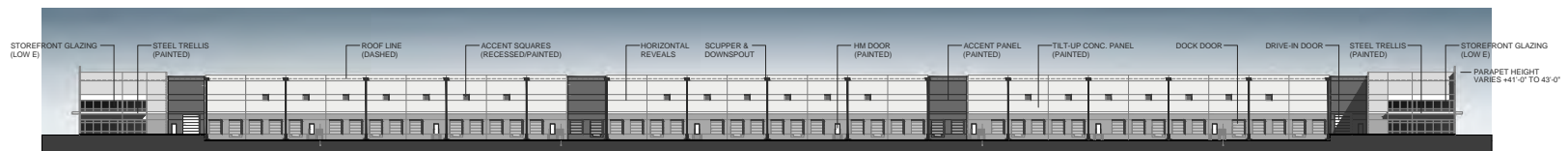
East Elevation (State Route 427)
