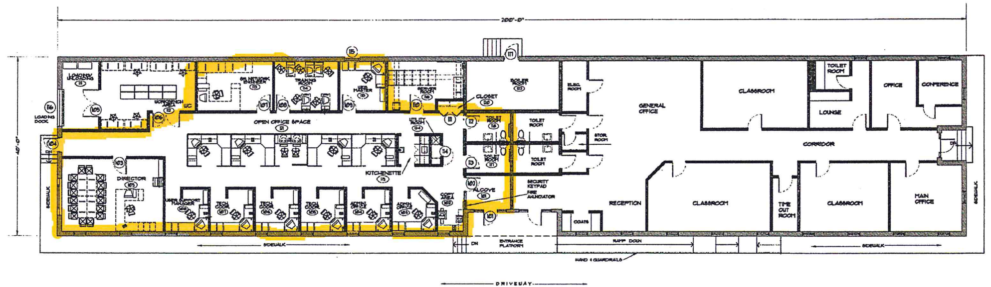
1 FIRST FLOOR PLAN A101
