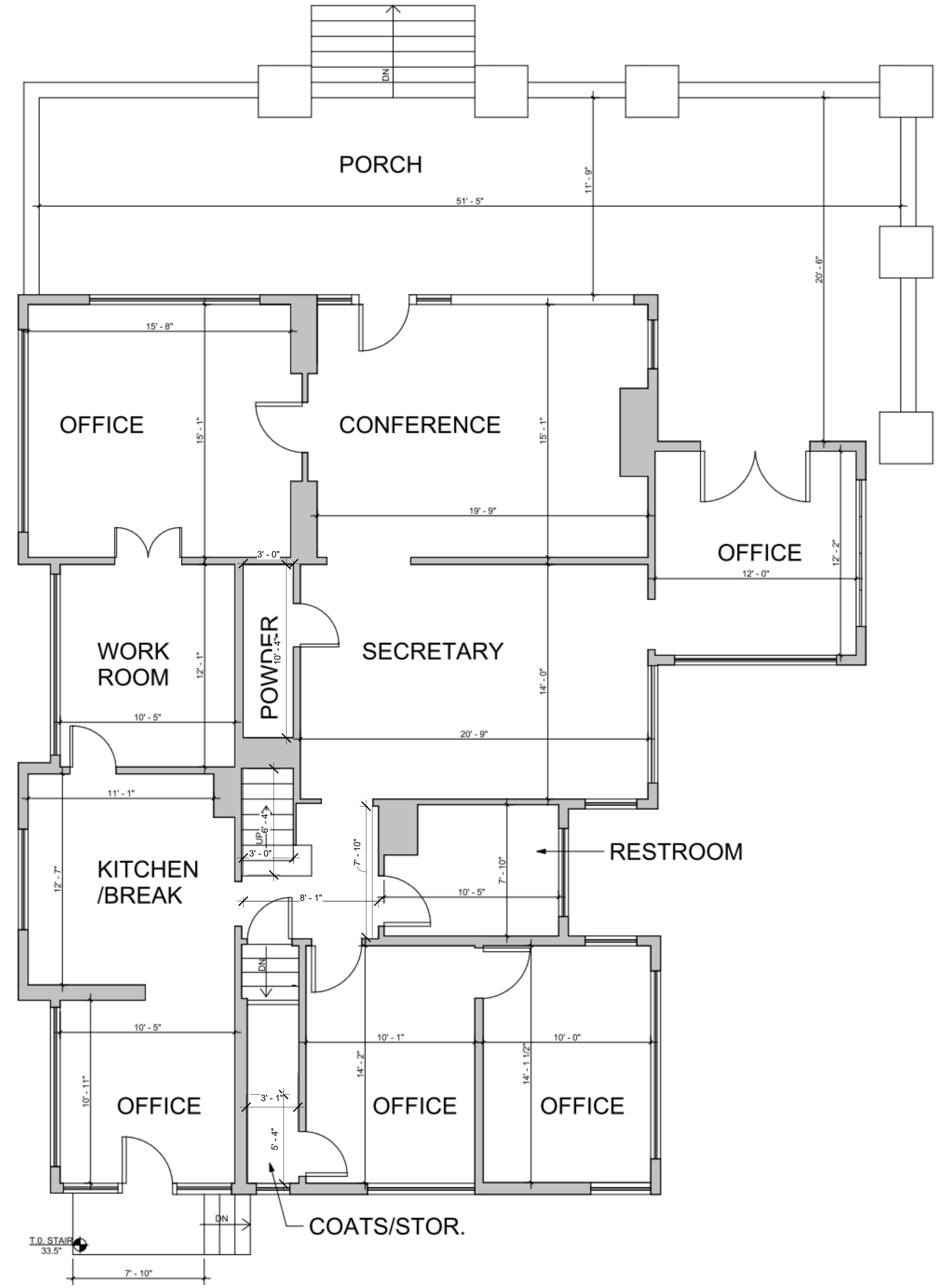
A FIRST FLOOR PLAN 1/4" = 1'-0"
