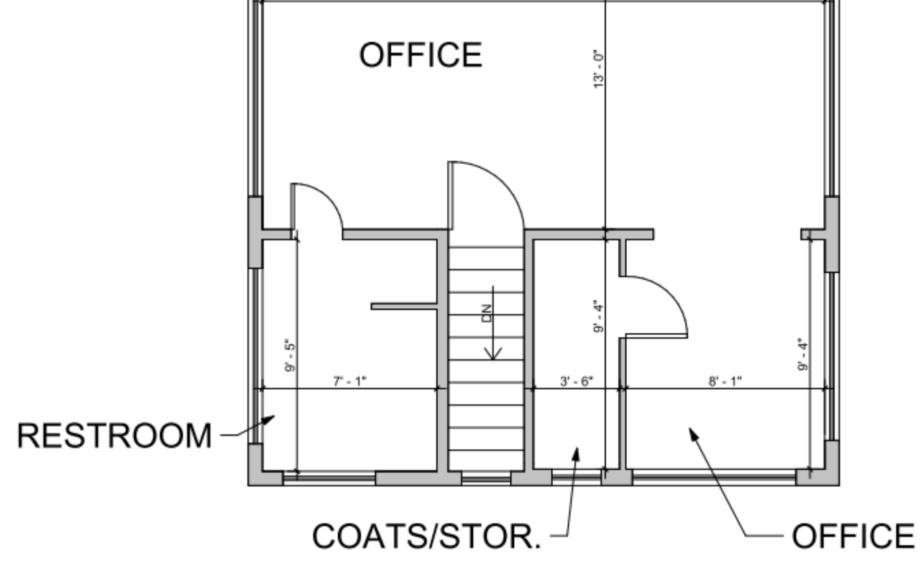
C SECOND FLOOR PLAN 1/4" = 1'-0"
