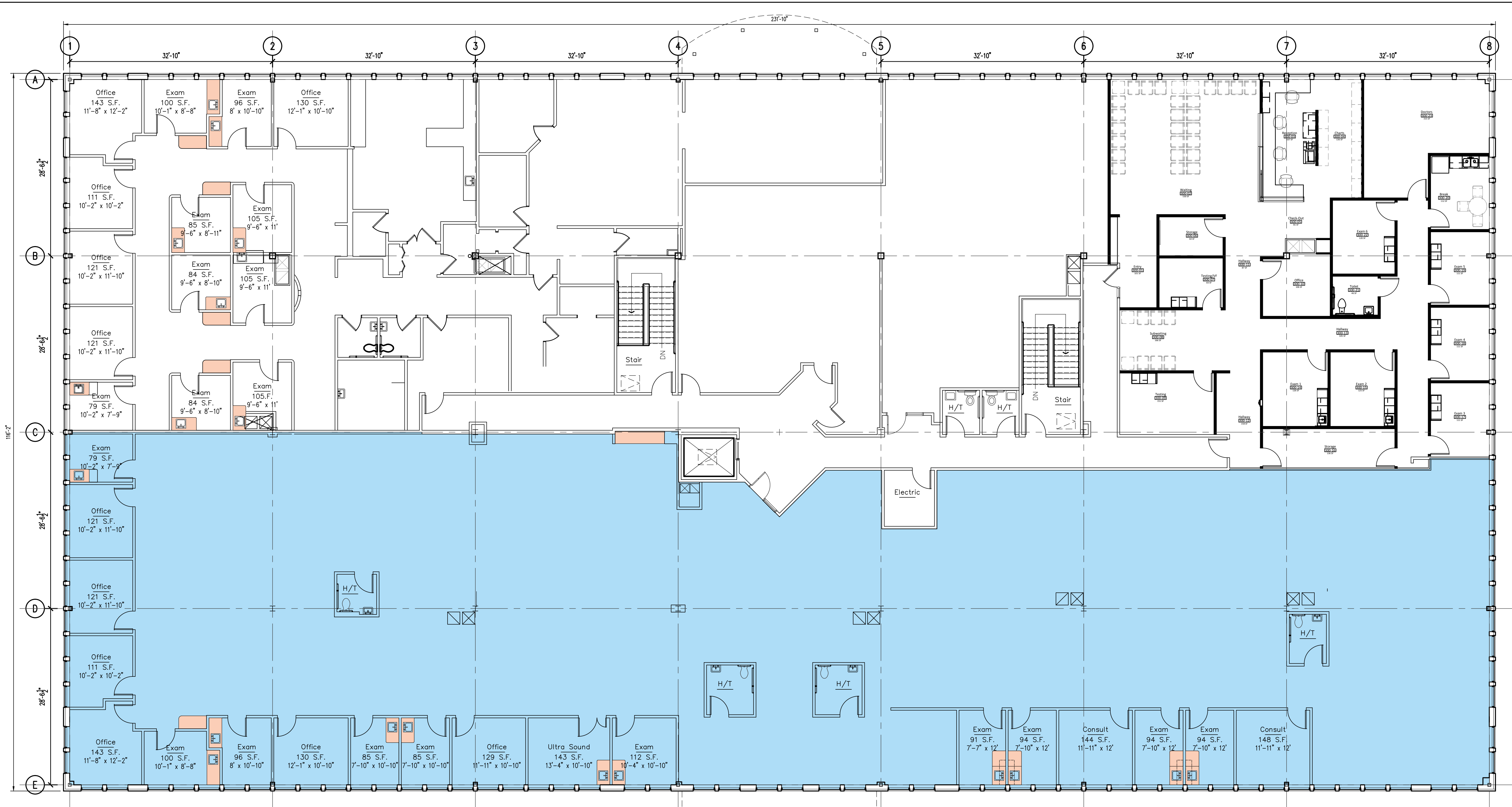
1 Revised Third Floor Plan A103 SCALE: 1/8"=1'-0"
