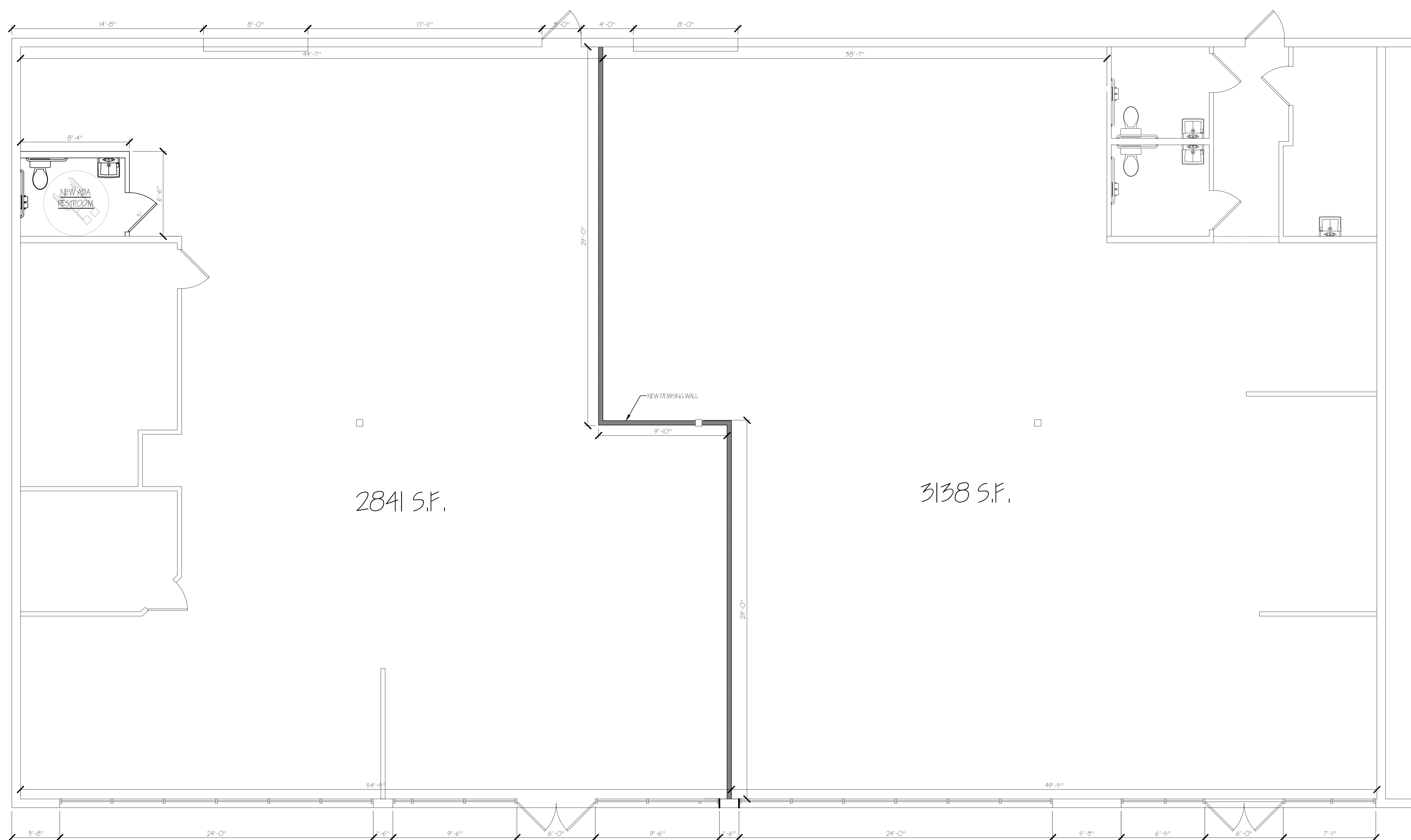
PROPOSED FLOOR PLAN SCALE: 1/4" = 1'-0"
