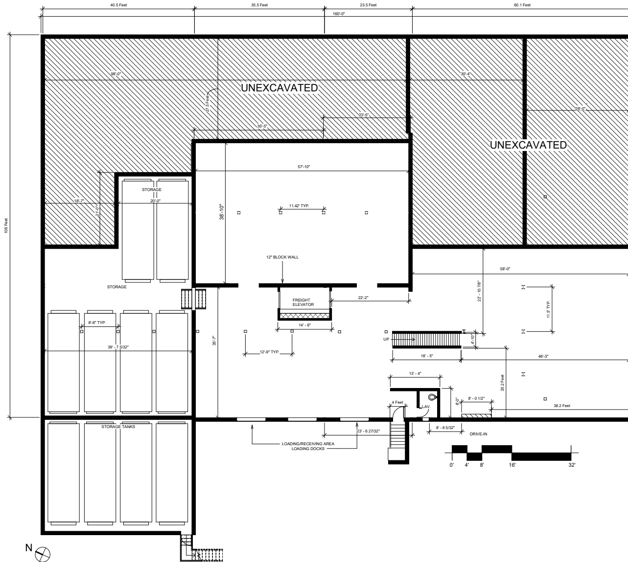
LOWER LEVEL FLOOR PLAN
