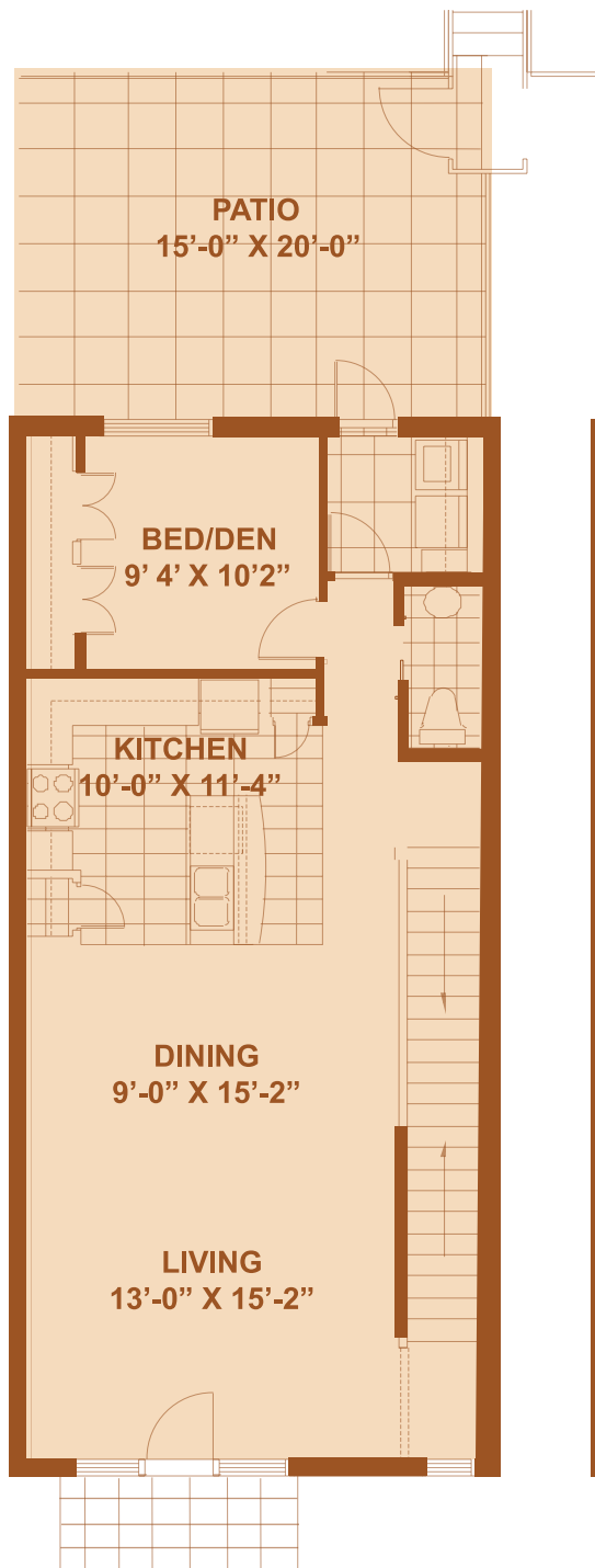
SECOND FLOOR 900 S.F.
