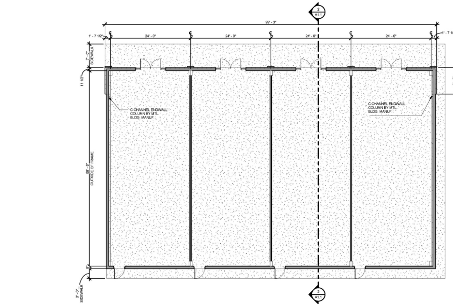
① FINISH SLAB 1/8" = 1'-0"
