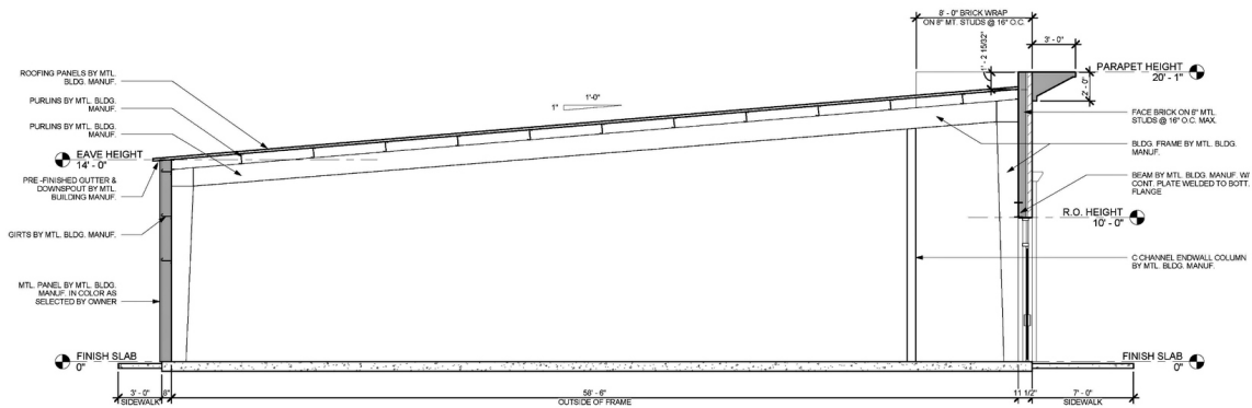
② Section 1 1/4" = 1'-0"
