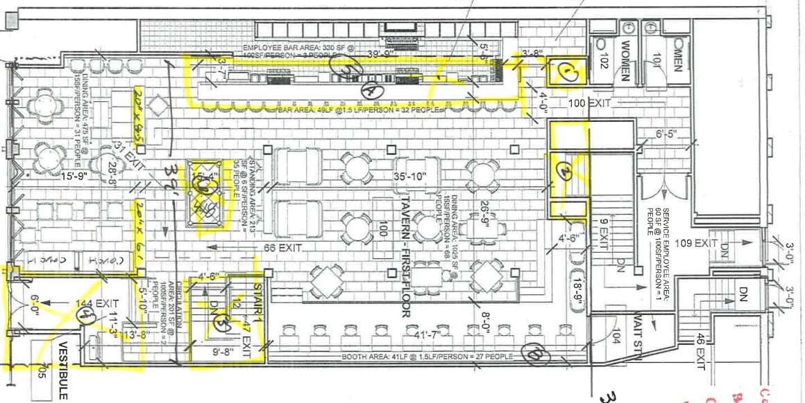
1 FIRST FLOOR OCCUPANCY PLAN 3/32" = 1'-0"
