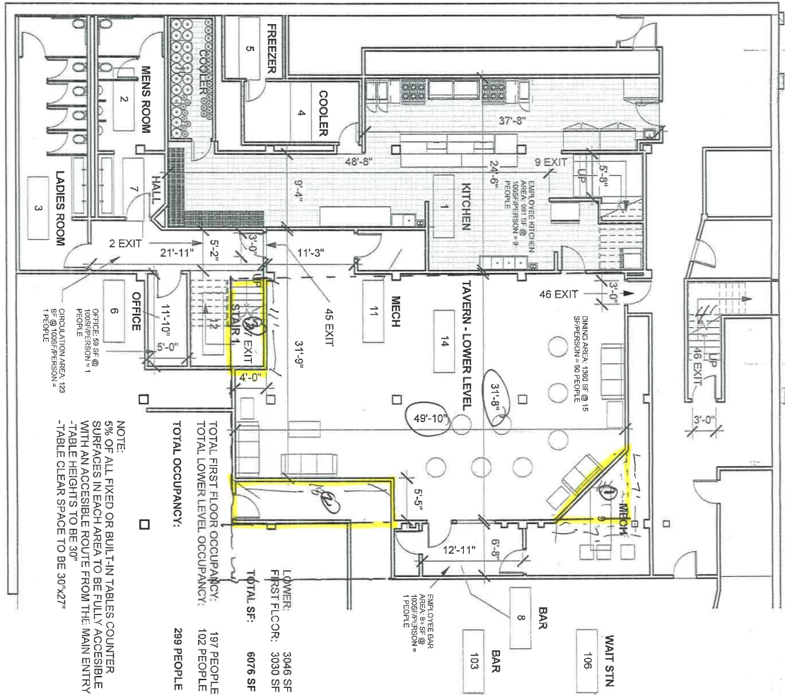
2 LOWER LEVEL OCCUPANCY PLAN 3/32" = 1'-0"
