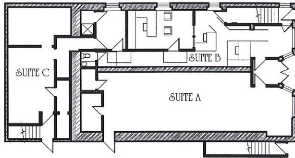
BUILDING GROUND FLOOR PLAN
