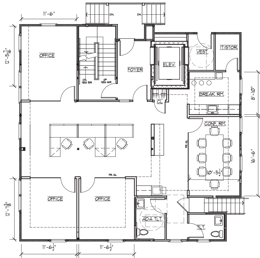
FIRST FLOOR: PRE-BUILT OFFICE PLAN
