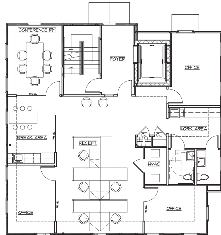
SECOND FLOOR: PRE-BUILT OFFICE PLAN
