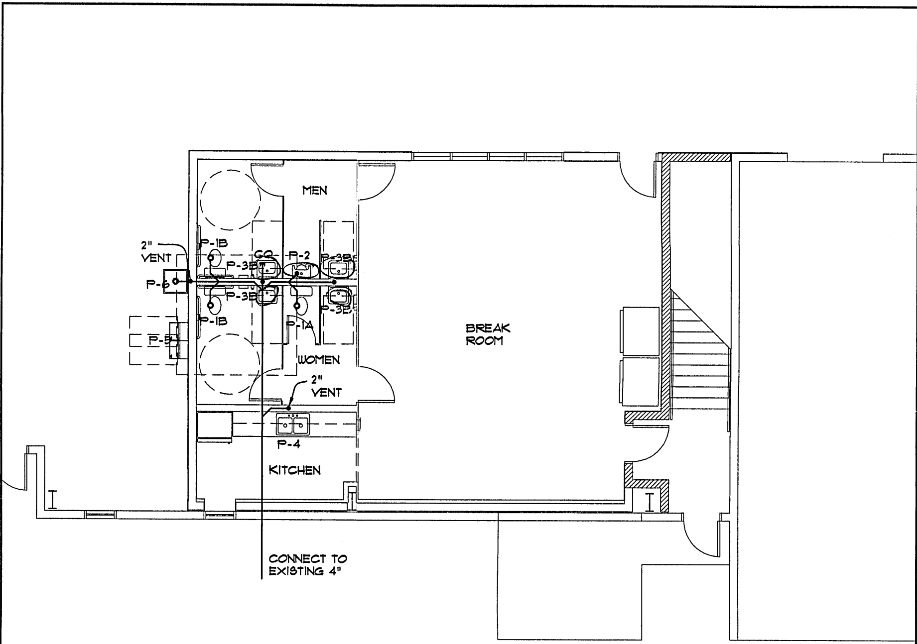
ENLARGED PLAN 'B' SCALE: 1/8"=1'-0"
