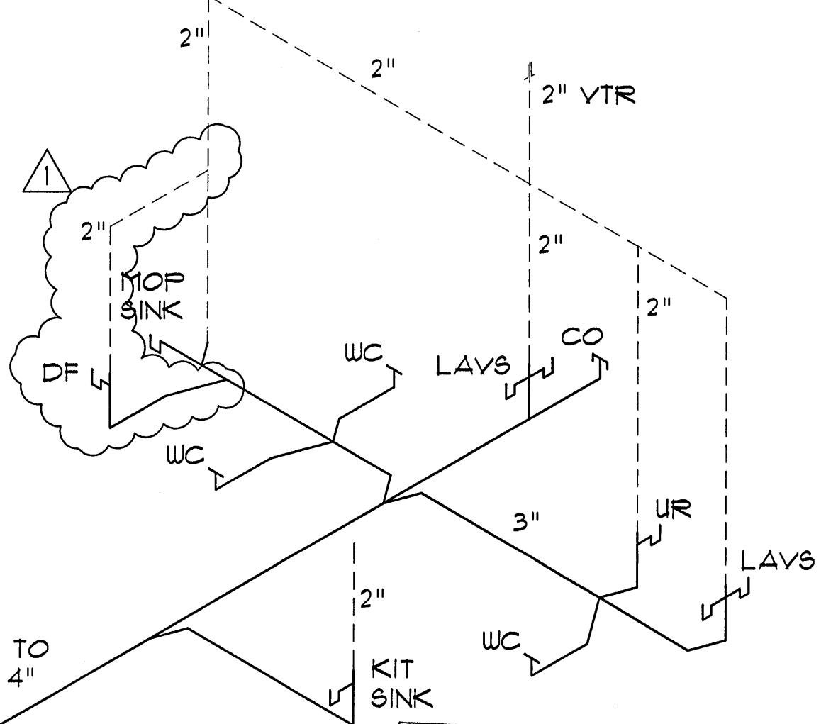
PLUMBING RISER (PLAN 'B' AND 'E') NOT TO SCALE
