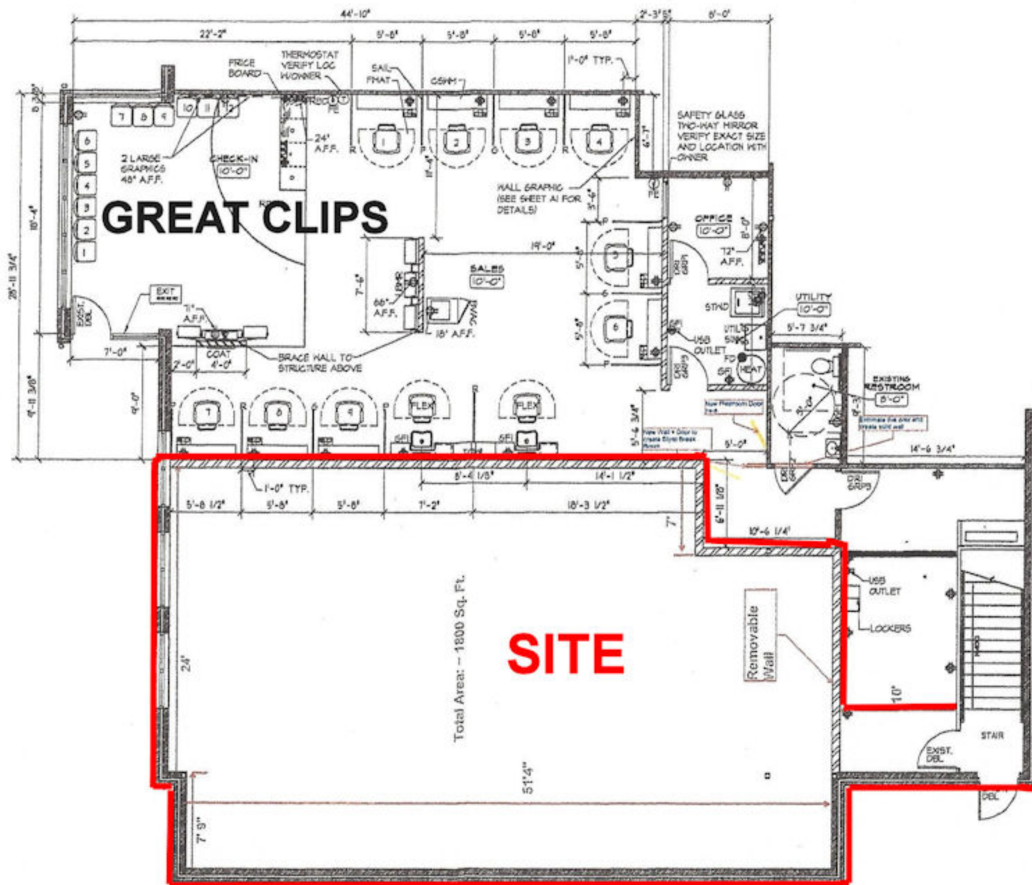
FLOOR PLAN 1/4" = 1'-0"
