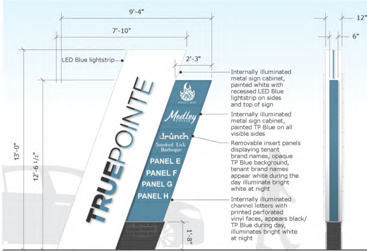
Elevation - Primary monument sign
