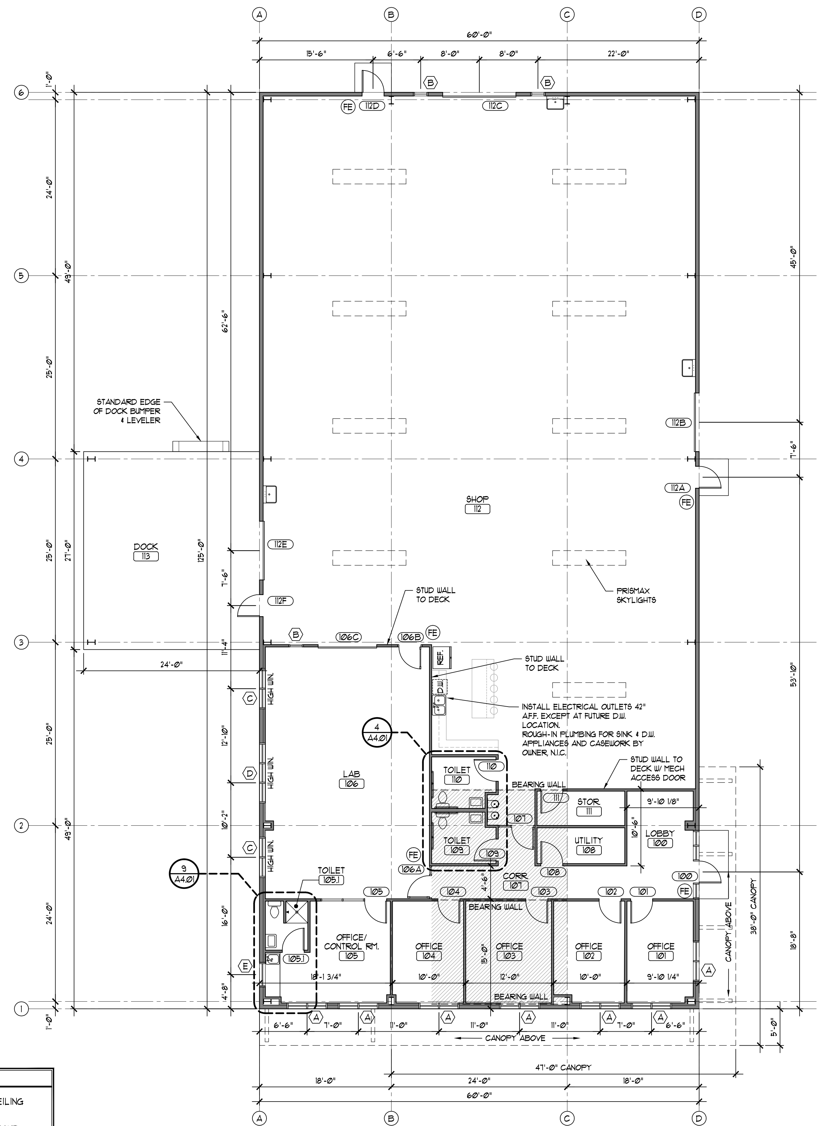
1 FLOOR PLAN SCALE 1/8" = 1'-0"
