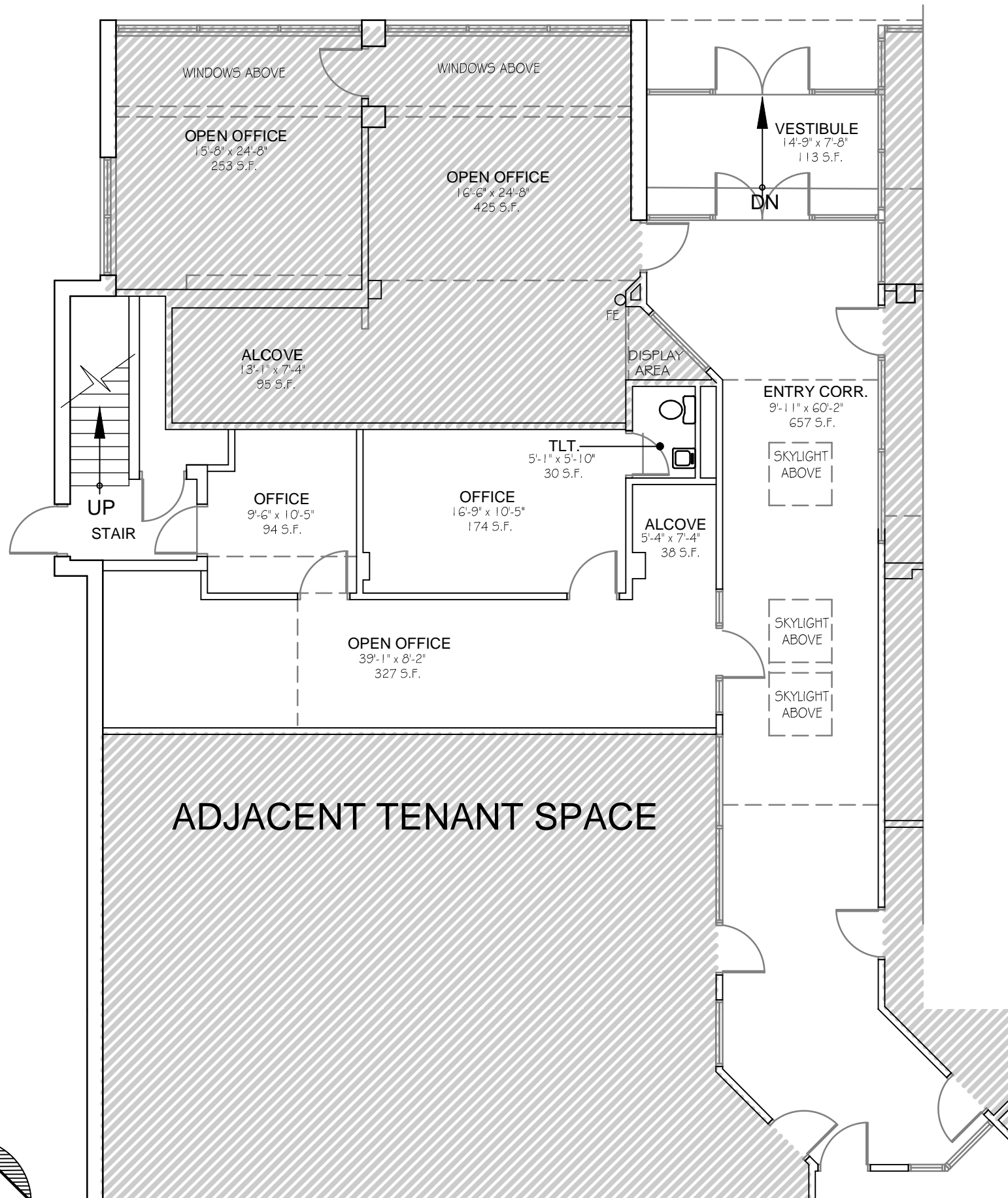
1 FLOOR PLAN - FIRST FLOOR - SUITE 103 SCALE: 1/16" = 1'-0" AUGUST 19, 2016 728 G.S.F. 660 S.F. NET USABLE AREA
