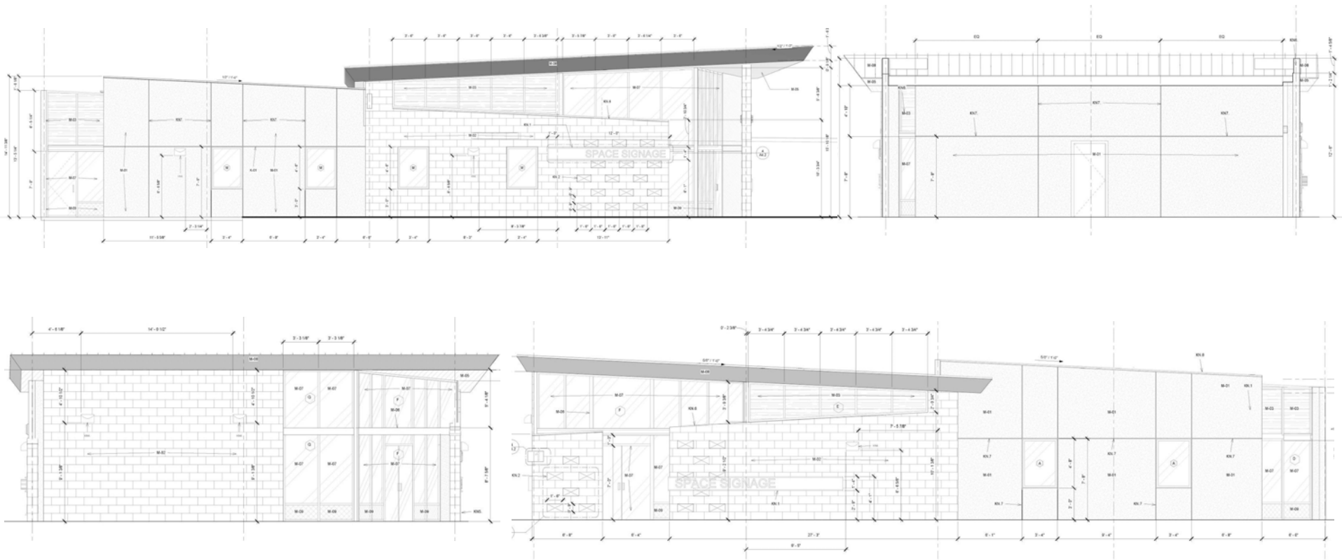
OPTION 1 - ELEVATIONS
