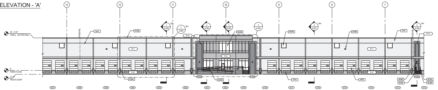
3 PARTIAL NORTH ELEVATION - 'B' A-201 1/16" = 1'-0"
