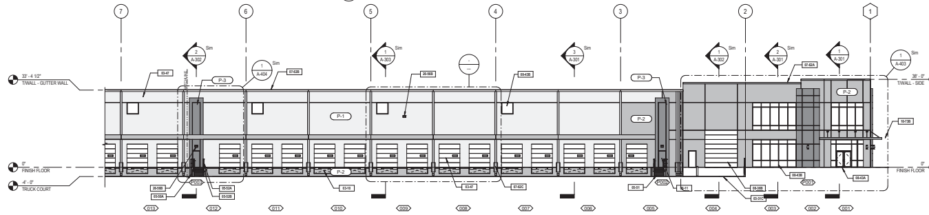
4 PARTIAL NORTH ELEVATION - 'C' A-201 1/16" = 1'-0"
